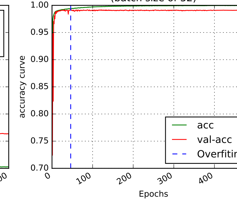
(a) ResNet (500) accuracy curve (batch size of 32)
