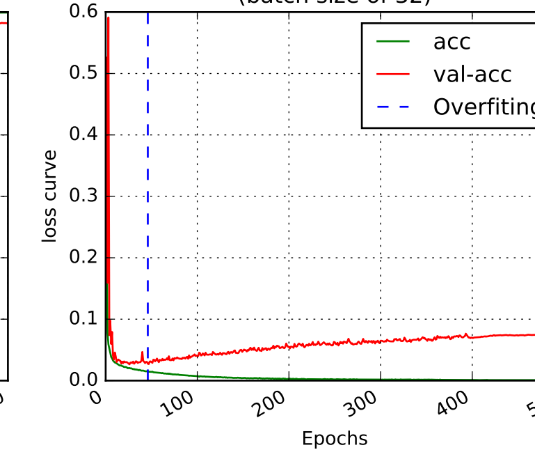
(b) ResNet (500) loss curve (batch size of 32)
