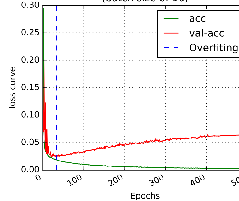
(b) ResNet (500) loss curve (batch size of 16)
