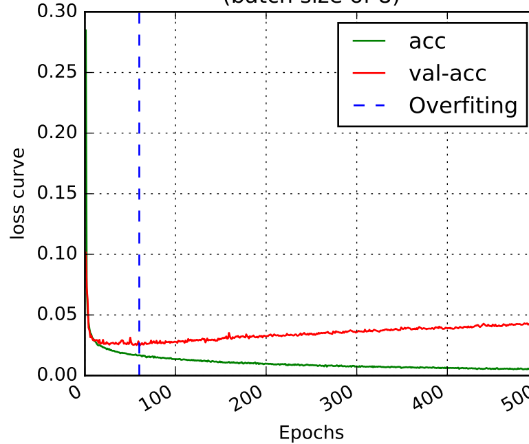
(b) ResNet (500) loss curve (batch size of 8)
