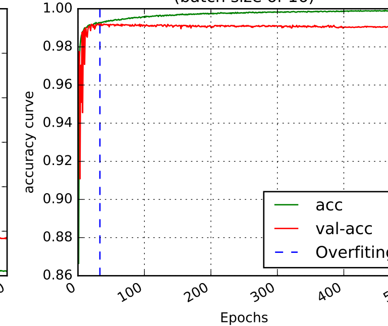
(a) ResNet (500) accuracy curve (batch size of 16)
