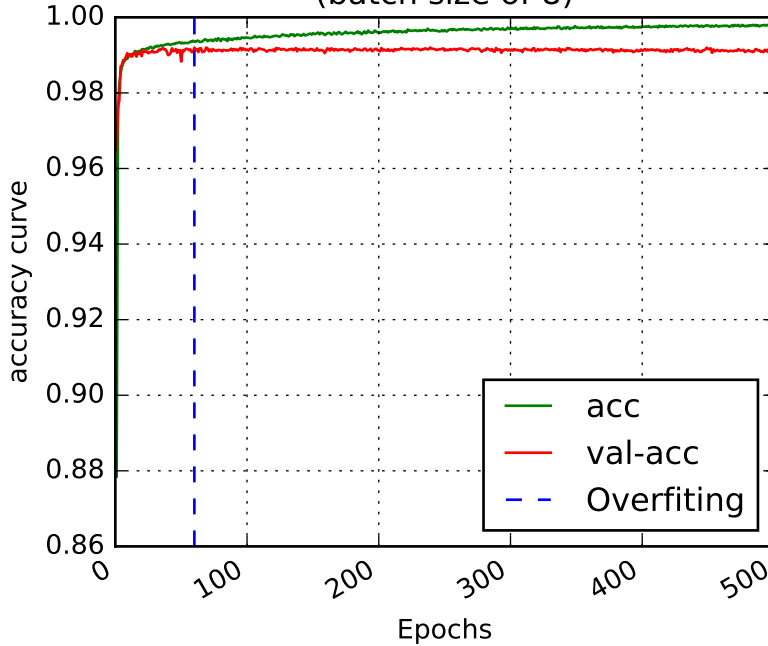
(a) ResNet (500) accuracy curve (batch size of 8)
